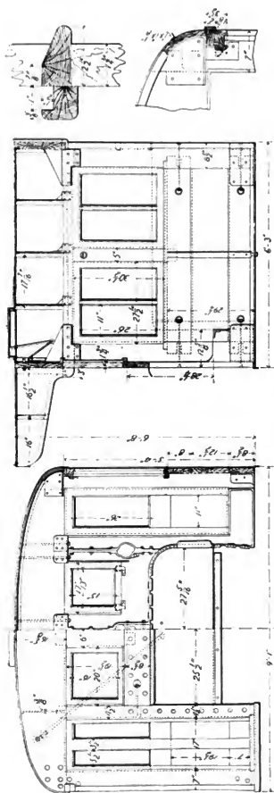
Figs. 2814-2817. Cab for Four-Wheel (0-4-0) Switching Locomotive, Pennsylvania Railroad.
